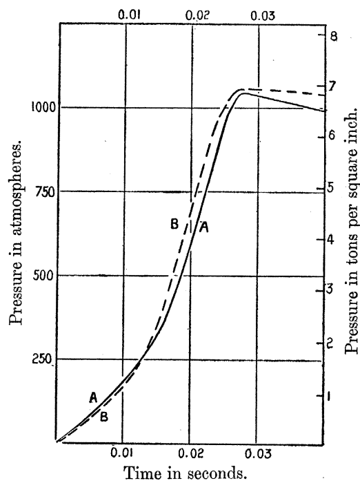
Fig. 9. Comparison of the effect of ignition by oxyhydrogen and gunpowder. Cordite of 0·175 inch diameter in a cylindrical enclosure; charge uniformly distributed; gravimetric density 0·1; A, fired with oxyhydrogen gas; B, fired with fine-grained powder.
