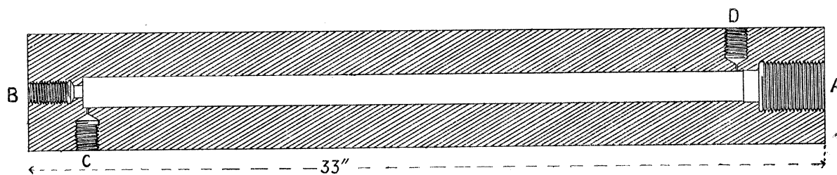
Fig. 6. Cylindrical enclosure.
