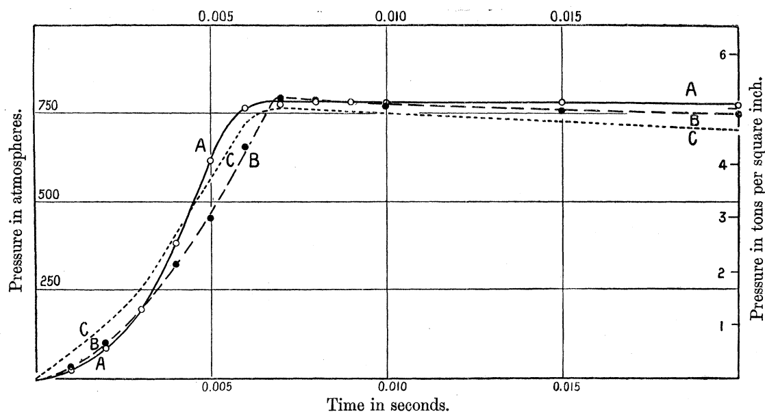
Fig. 14. Showing the rate of rise of pressure for cordite of the smallest diameter. Diameter 0·035 inch (0·89 millim.).
