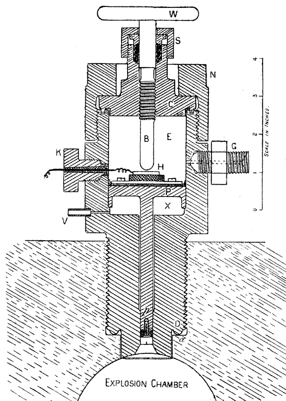
Fig. 1. Explosion gauge. (Maximum pressure indicator.)
